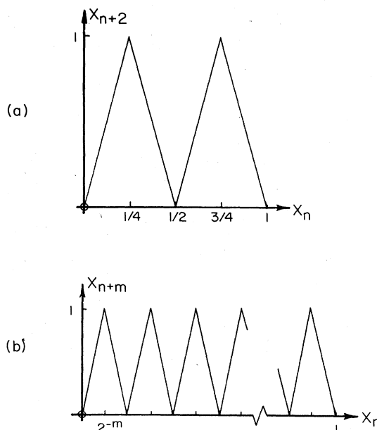
FIG. 4. (a) x_{n+2} vs x_n for F_1 with a=1 . (b) x_{n+m} vs x_n for F_1 with a=1 (the length along the x_n axis is expanded).
