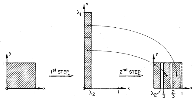
FIG. 12. Map motivating Eq. (3.9). The illustrated map may be represented analytically as y_{n+1} = 3y_n \bmod 1 , x_{n+1} = \lambda_2 x_n + y_n - y_{n+1}/3 .
