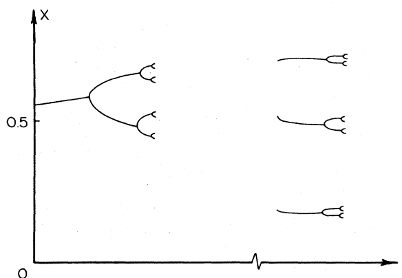
FIG. 7. Summary diagram for some of the bifurcations of F^{(2)} . The scale about the period 3 \times 2^k cycles has been greatly expanded.
