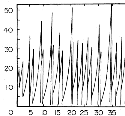
FIG. 18. a_1 vs t for \gamma = 15 .
