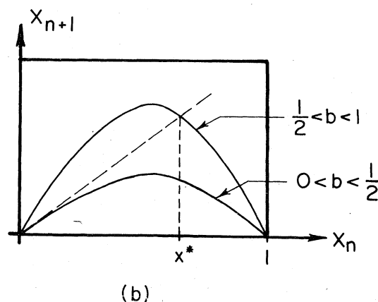
FIG. 1. (a) Map F_1 [Eq. (2.2)], and (b) the map F_2 [Eq. (2.3)].
