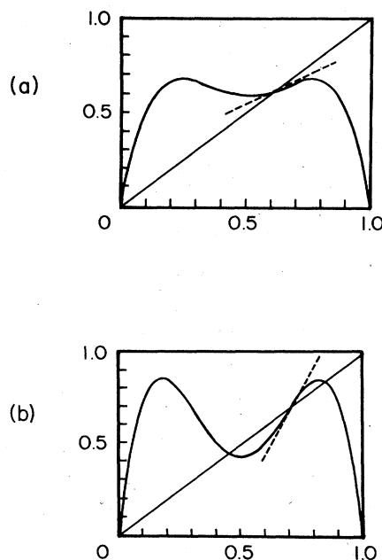
FIG. 5. x_{n+2} vs x_n for F_2 with (a) b = 0.678 and (b) b = 0.854 . The dashed lines are the slope at x = x^* . The intersections of x_{n+2} = x_n with x_{n+2} - F_2^{(2)}(x_n) are e > x^* > f .
