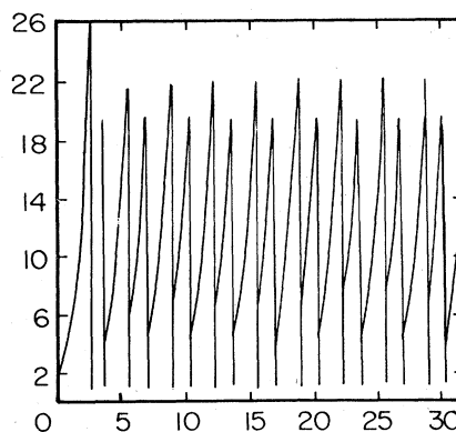
FIG. 17. a_1 vs t for \gamma = 9 .
